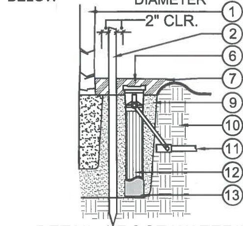
DETAIL-1 ROOT WATERING SYSTEM
